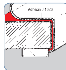
Adhesin J 1626
